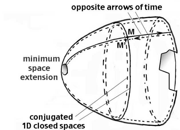
Fig.35 : 2D didactic image of Janus model without singularity
